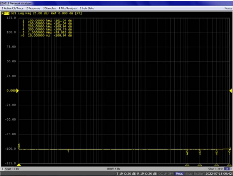
CM 0301M Broadband Current Monitor s21 curve
