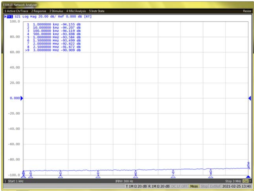
CM 03203M Broadband Current Monitor s21 curve
