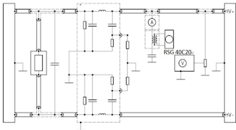
ISO 7637-4, B-wave HV+ line-to-ground:
