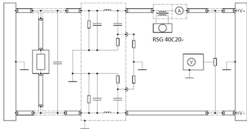
ISO 7637-4, B-wave line-to-line
